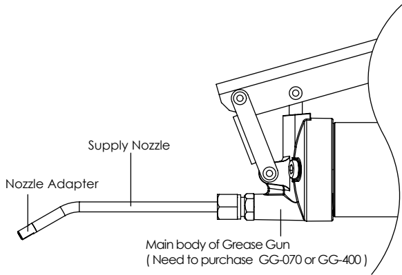
Greasing Diagram
