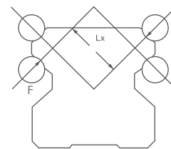
X-Type Arrangement
